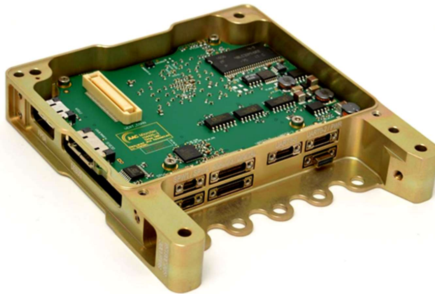
Figure 2.1 The Sirius OBC product without lid.
