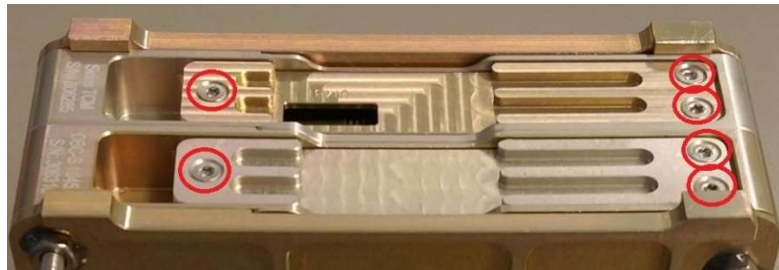
Figure 2.4 Countersunk screws for debug hatch covering the JTAG and Debug connectors.
