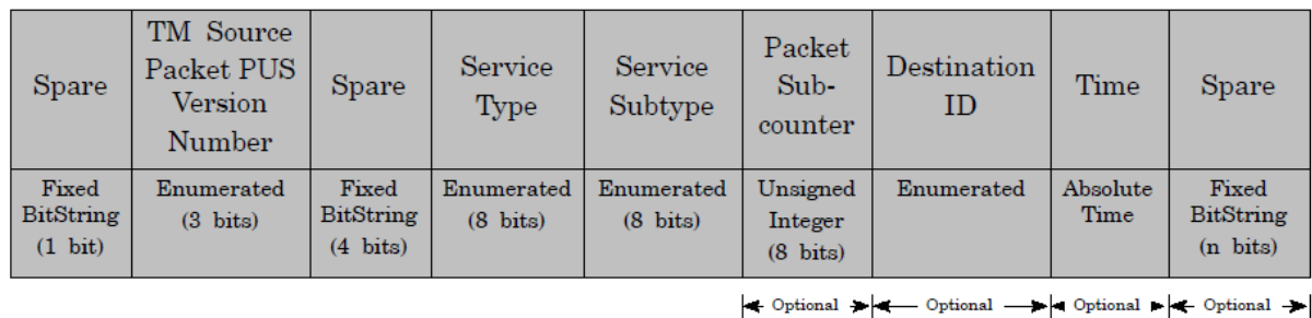
Figure 10-11 Data Field Header
