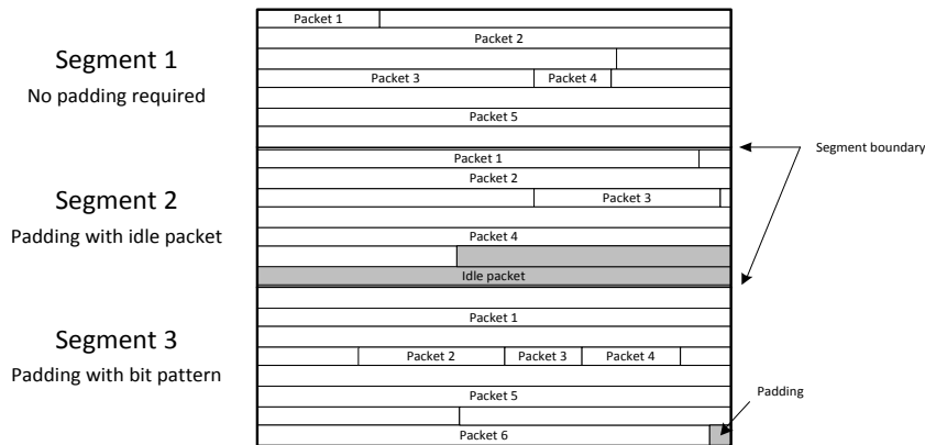
Figure 7-6 Illustration of packet placement inside segments with different padding (marked in grey)
