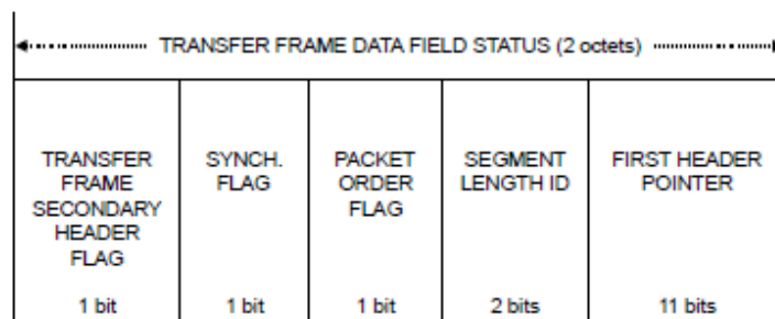
Figure 11.12 - Transfer Frame Data Field Status
