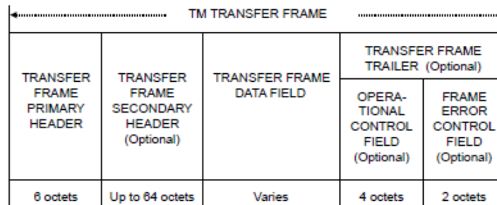
Figure 11.10 - Telemetry Transfer Frame
