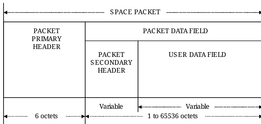
Figure 11.6 - CCSDS Space Packet (reproduced from [RD18])
