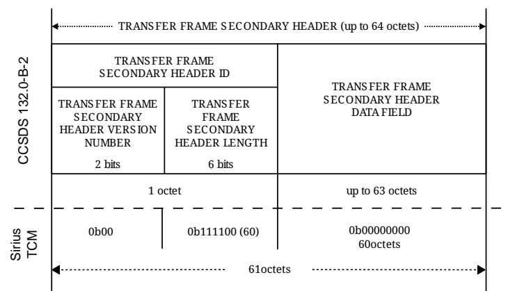
Figure 11.13 - Transfer Frame Secondary Header
