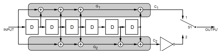
Figure 11.9 - Convolutional Encoder Block Diagram
