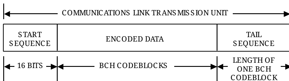
Figure 11.1 - CLTU (reproduced from [RD17])
