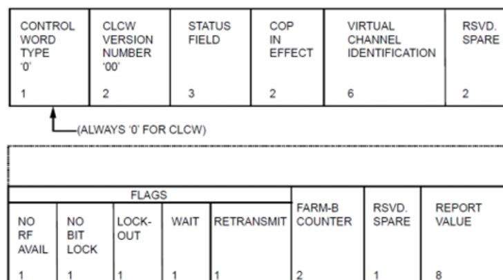
Figure 11.14 - Command Link Control Word
