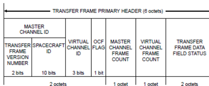
Figure 11.11 - Telemetry Transfer Frame Primary Header
