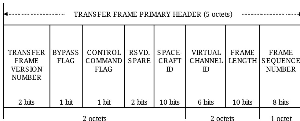
Figure 11.4 - TC Transfer Frame Primary Header (reproduced from [RD13])
