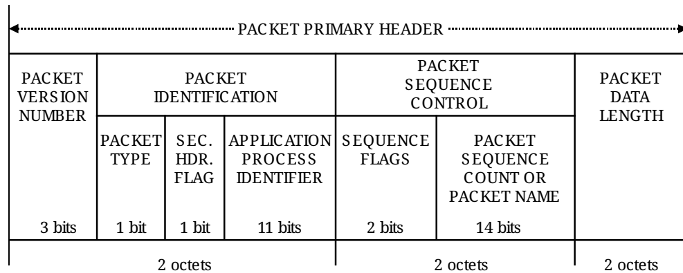
Figure 11.7 - CCSDS Space Packet Primary Header (reproduced from [RD18])
