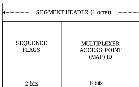
Figure 11.5 - TC Segment Header (reproduced from [RD13])
